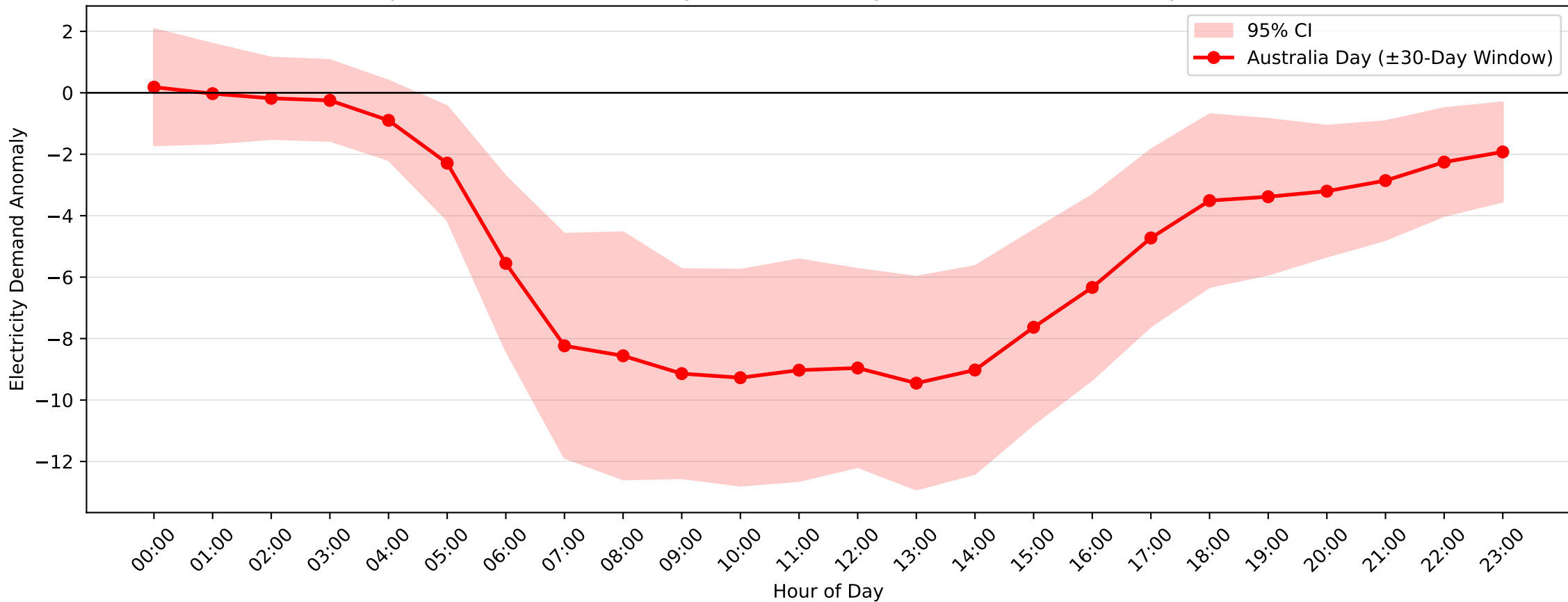
Milperra Demand Anomaly: Australia Day (2004-2017, \pm 30 -Day Window)
